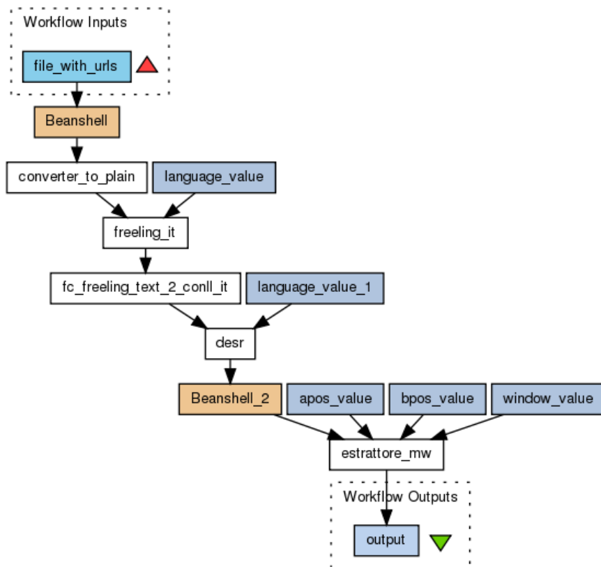
Figure 2: MWE lexicon extractor from text
