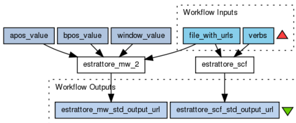
Figure 1: Dependency parsed 2 Italian MWE and SCF acquisition workflow
